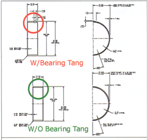
Figure 3 An example of connecting rod bearings that are now being manufactured without the tab. Bearing manufacturing print courtesy of Federal-Mogul.
